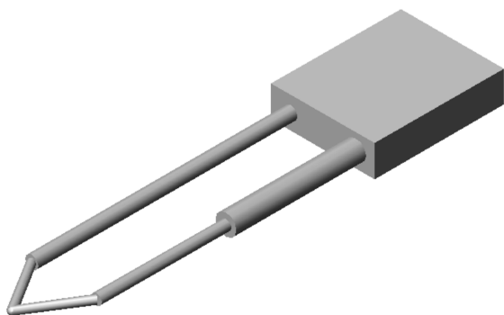
Fig. 2b. A cavity composed of two pipes, pipe 1 and pipe 2, connected in parallel. At the left side of these pipes runners are replaced for a thick cavity of two square plates to deliver resin to both sides of pipes.
