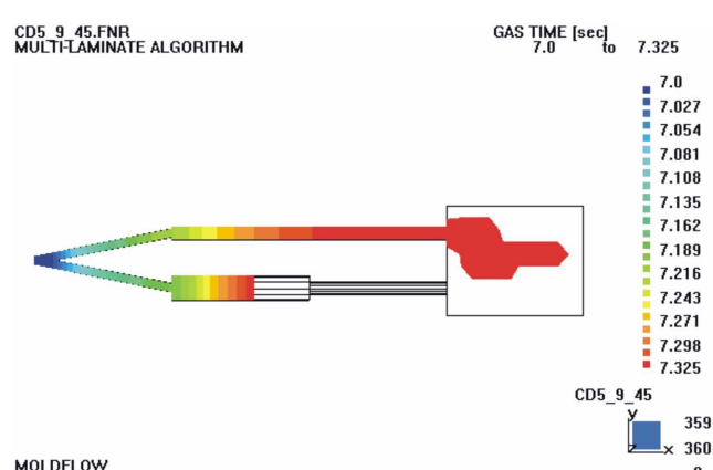
Fig. 19. The geometry is similar to Fig. 8 except that diameter of pipe 21 is 9 mm. Instead of a thick cavity of two square plates, branching runners with diameter of 3 mm are attached at the left hand side to deliver resin to pipes at both upper side and lower side.
