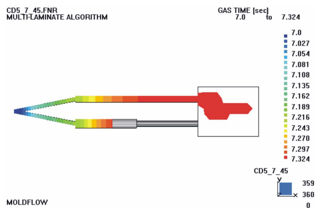
Fig. 17. The geometry is similar to Fig. 8 except that diameter of pipe 21 is 7 mm. Instead of a thick cavity of two square plates, branching runners with diameter of 3 mm are attached at the left hand side to deliver resin to pipes at both upper side and lower side.
