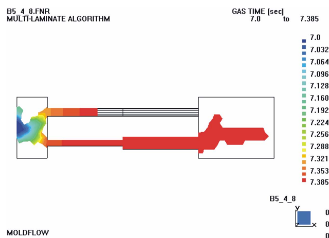
Fig. 7. The geometry is the same as Fig. 6 except that diameter of pipe 21 is 4 mm.
